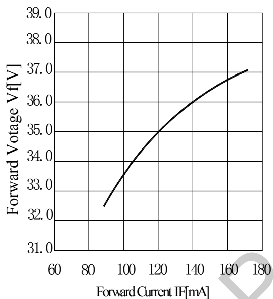
Forward Votage Vs. Forward Current
