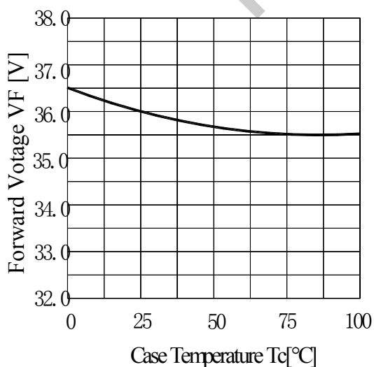
Case Temperature Vs. Forward Votage
